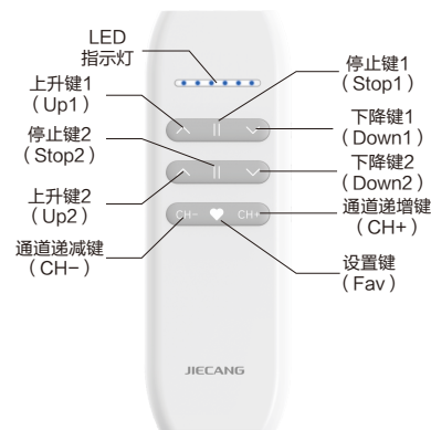
JCHR35W3A8—六通道双路
